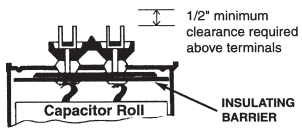
Normal Position of Protective Device
