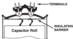
Position of Protective Device After Activation
