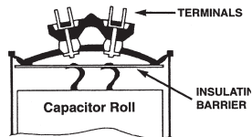
Position of Protective Device After Activation
