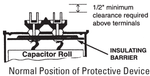
Normal Position of Protective Device
