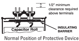
Normal Position of Protective Device
