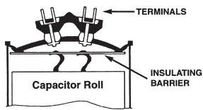
Position of Protective Device After Activation
