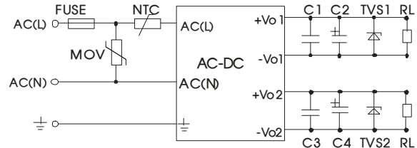
Fig. 4: LH20-10D series (Isolate Twin Output) typical application circuit
